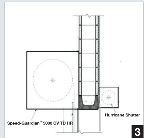
Hurricane Shutter Exterior Mount
