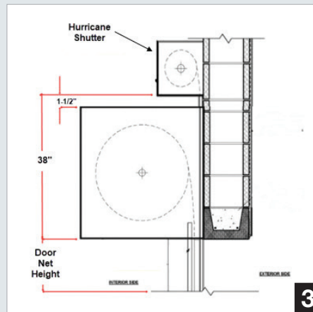
Hurricane Shutter Above Lintel Mount
